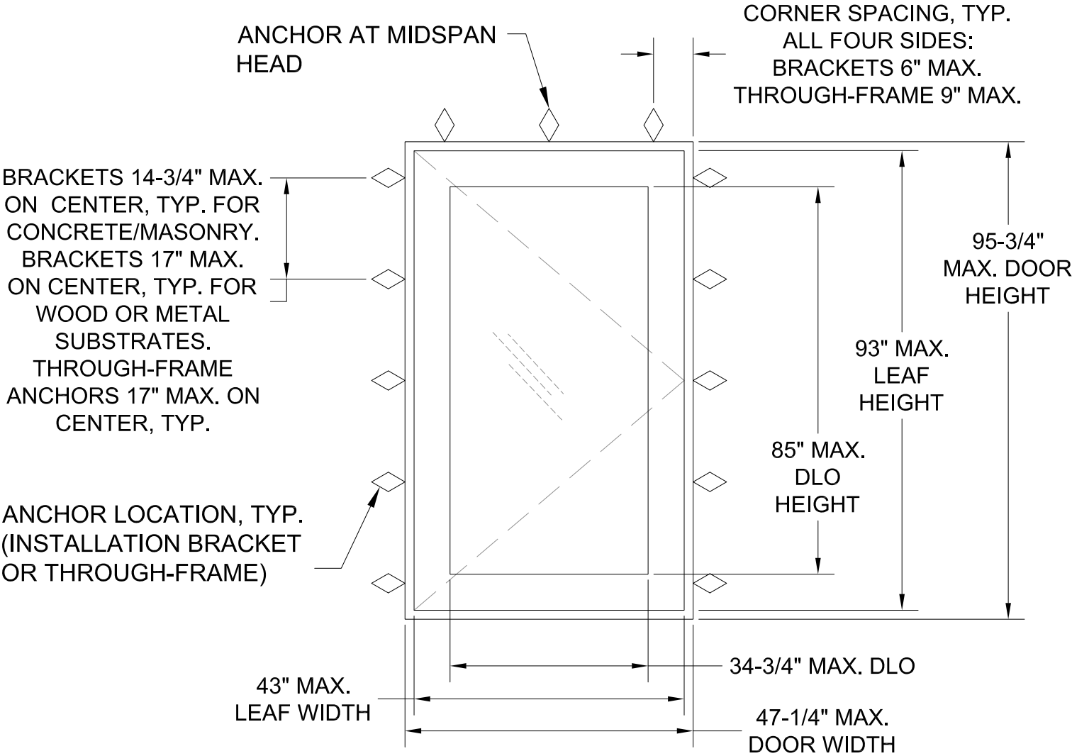
TYP. ELEVATION SEE DETAILS SHEET 2
